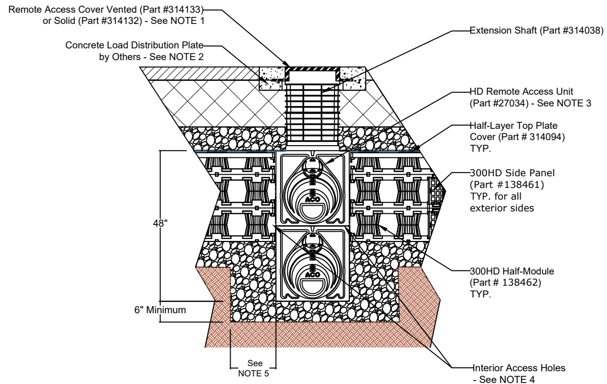
2.5 LAYER 300HD REMOTE ACCESS UNIT CROSS SECTION
