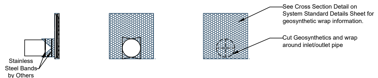
DETAIL A PIPE WRAP
